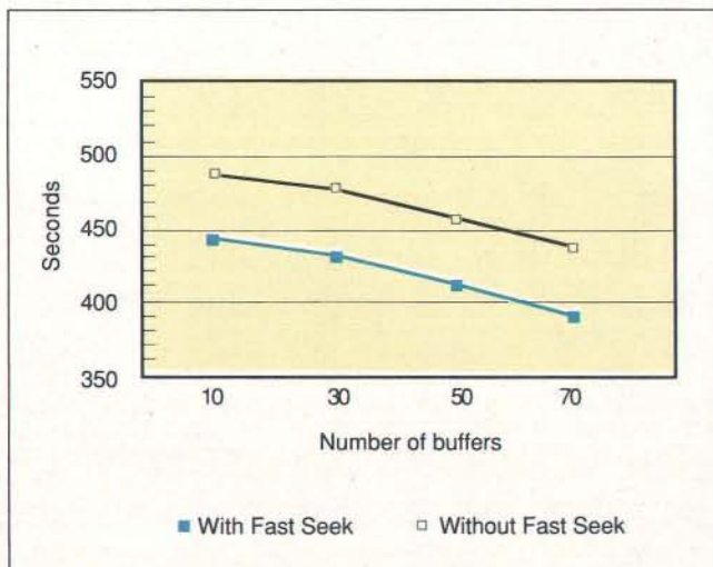
Figure 6: The performance improvements from using Fast Seek for random-sector reads and writes in the same test as for large buffers (12,800 random-sector reads and writes on a 256K-byte file).
